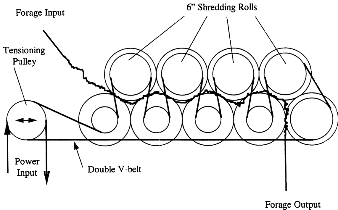
Figure 3. Schematic of Roughened - Roll Macerator
