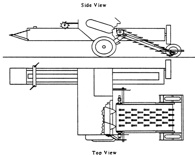
Figure 7: Belt-and-Time Pick-up for Forage Mats Mounted on Conventional Small Rectangular Baler.
