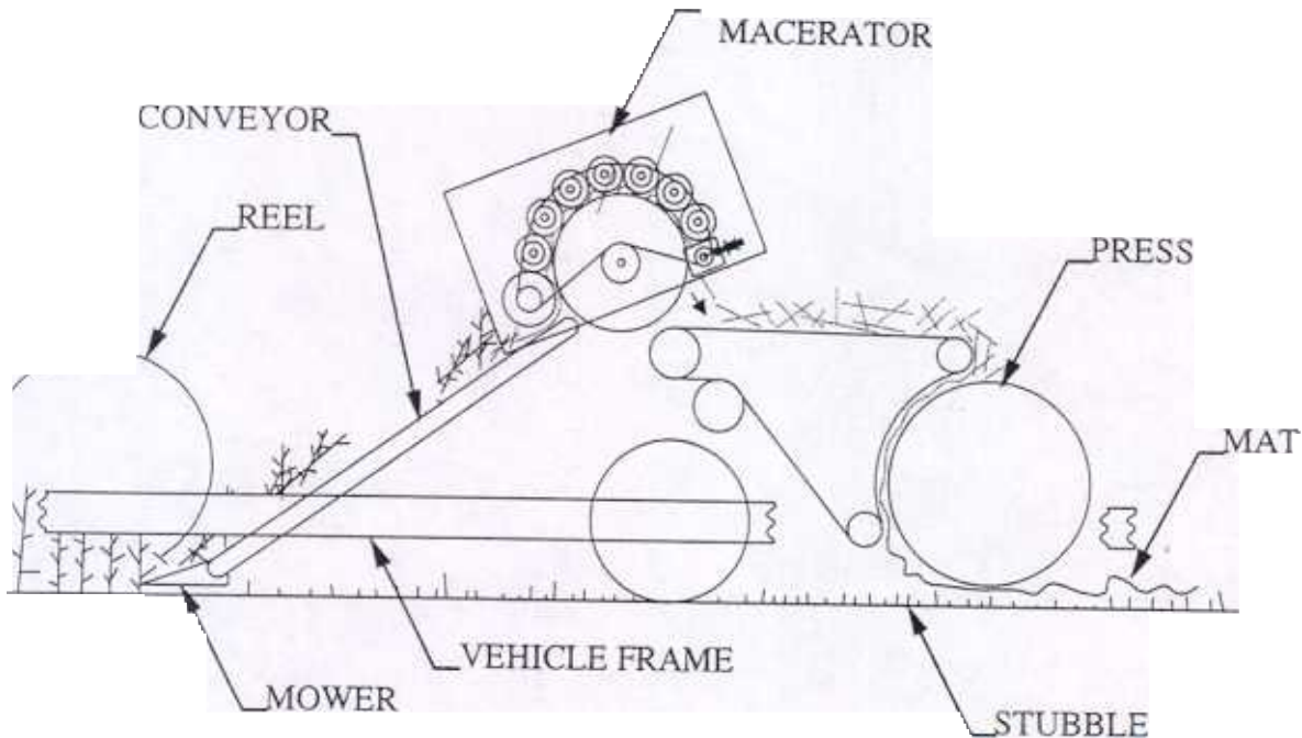
Figure 1. Schematic of the Original Wisconsin Prototype Mat Machine
