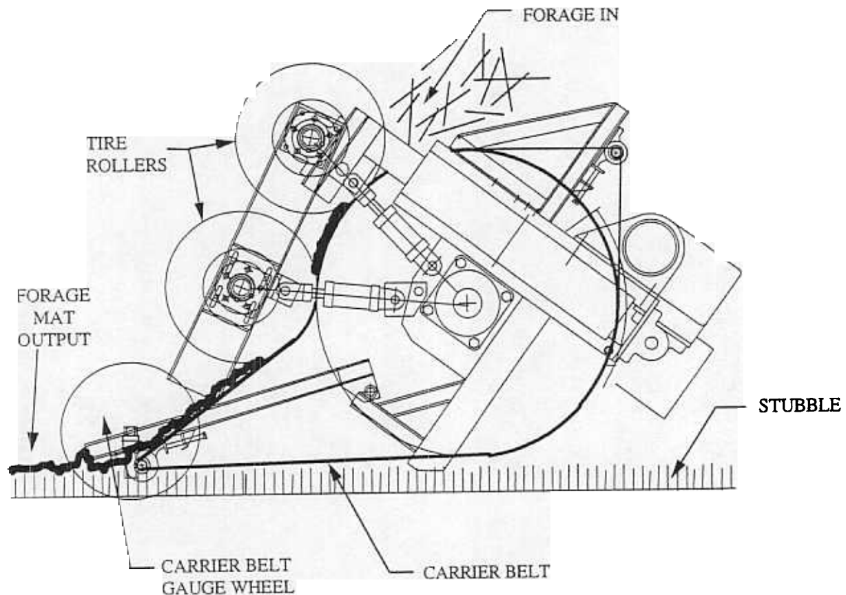
Figure 5. Press for Forming Macerated Forage Mats
