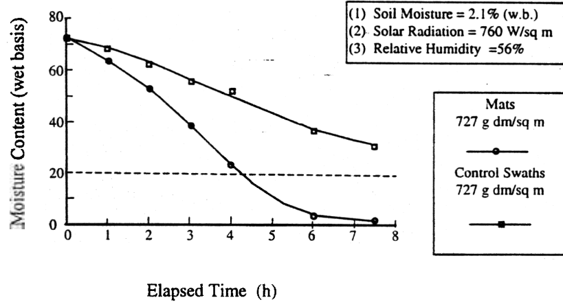
Figure 2. A Comparison of Drying Rates for Mat-Processed and conventionally Conditioned Alfalfa.
